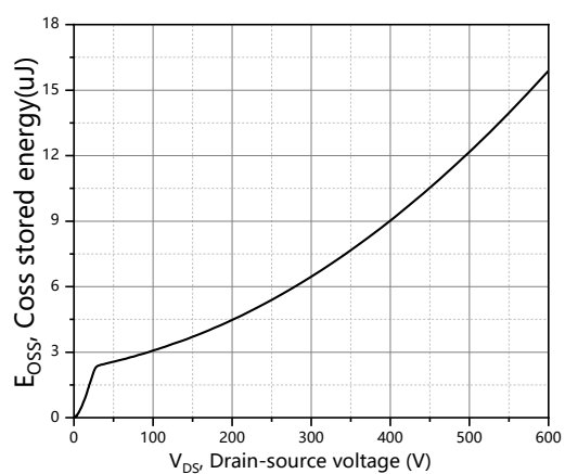
Figure 13. Typ. Coss stored energy
