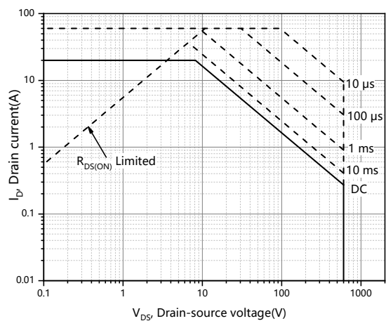
Figure 11. Safe operation area for T_C=25^\circ C
