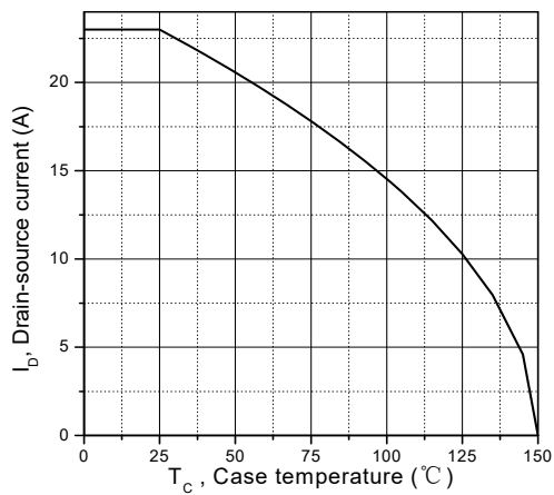
Figure 9. Drain current
