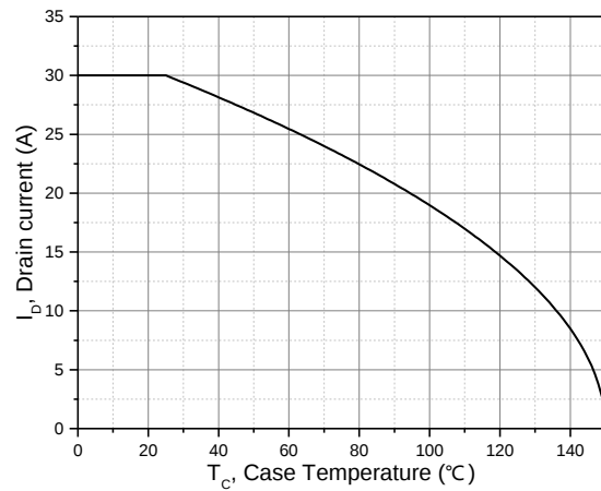
Figure 10. Drain current
