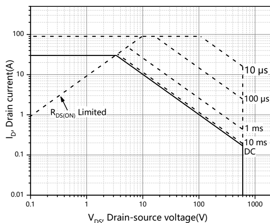
Figure 10. Safe operation area for T C =25 °C
