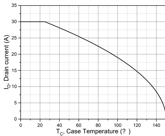
Figure 9. Drain current
