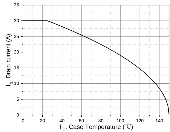
Figure 10. Drain current
