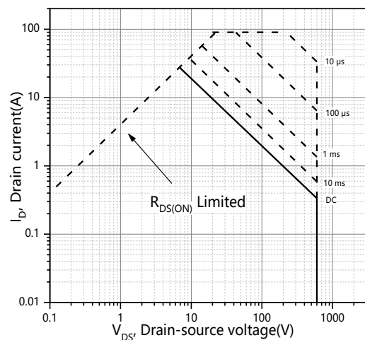
Figure 12. Safe operation area for T_C=25^{\circ}\text{C}
