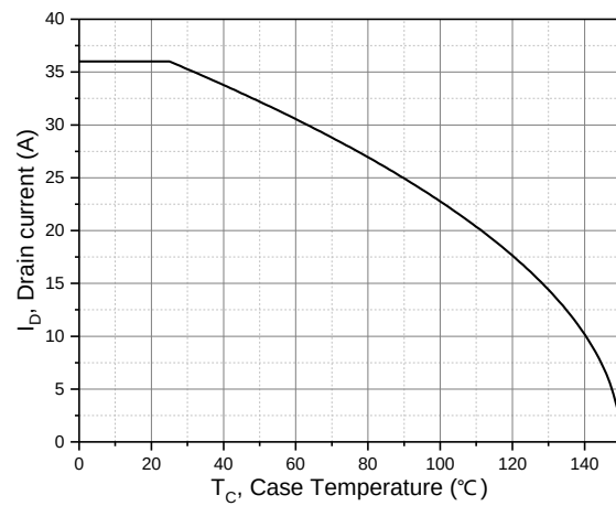
Figure 10. Drain current
