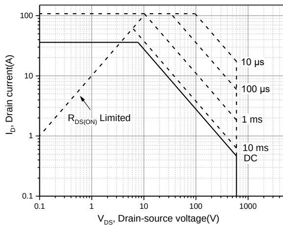
Figure 11. Safe operation area for TC=25 °C
