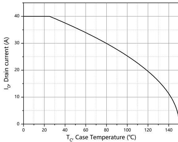
Figure 9. Drain current
