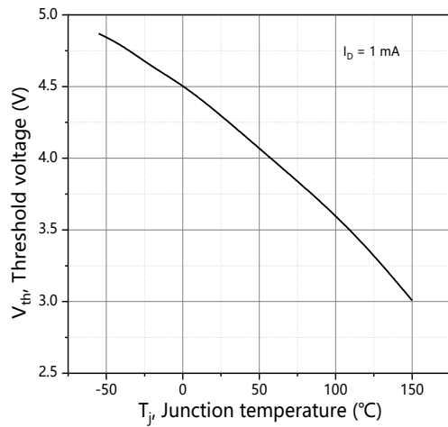
Figure 7. Threshold voltage
