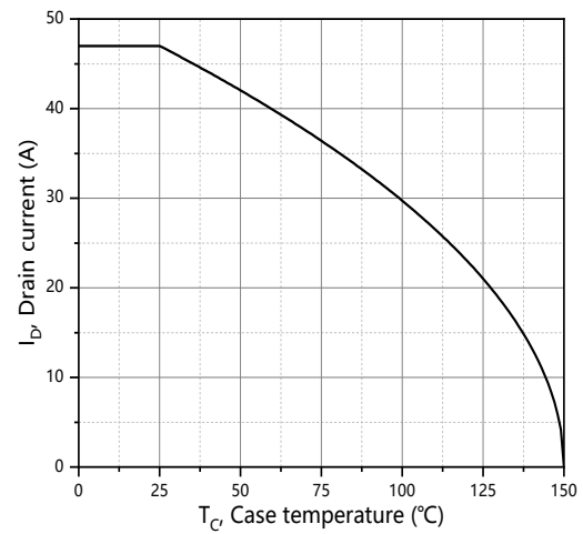
Figure 10. Drain current
