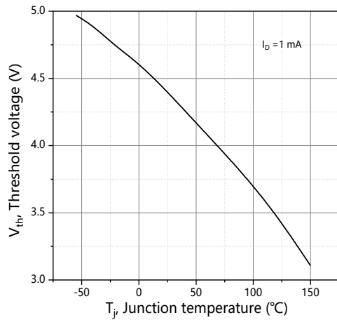
Figure 7. Threshold voltage
