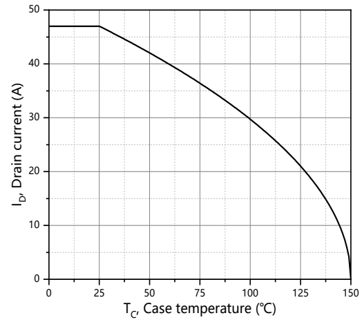
Figure 10. Drain current
