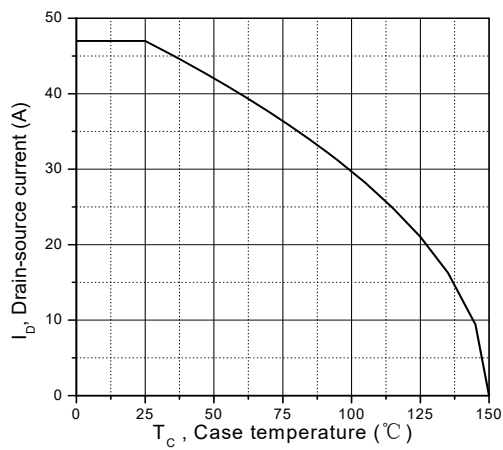
Figure 9. Drain current
