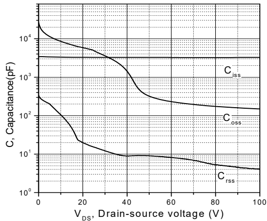
Figure 3. Typ. capacitances
