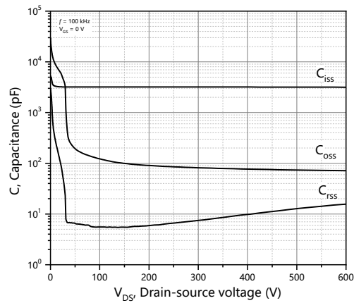
Figure 3. Typ. capacitances
