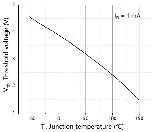
Figure 7. Threshold voltage
