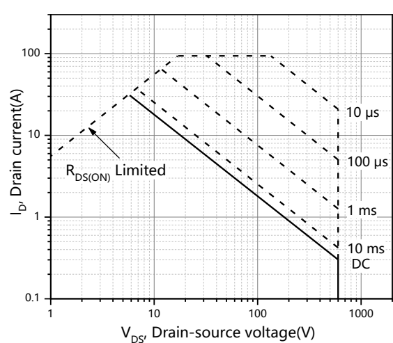
Figure 12. Safe operation area for T_c=25^{\circ}\text{C}
