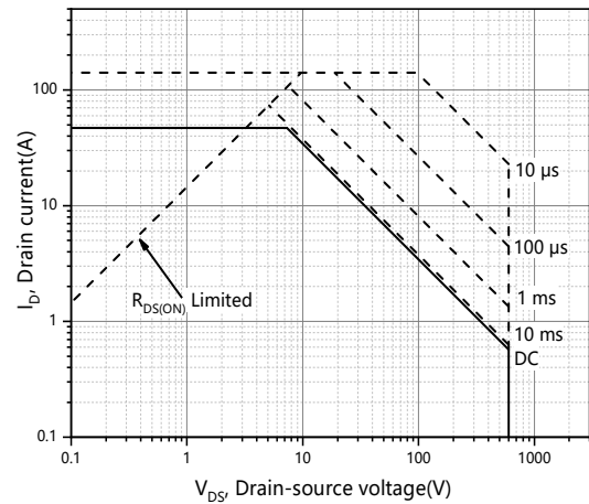
Figure 12. Safe operation area for T_C=25 °C
