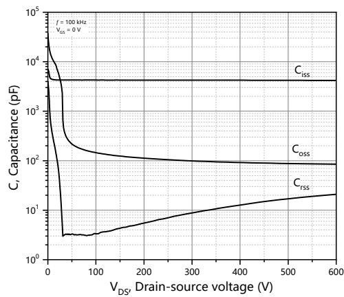
Figure 3. Typ. capacitances
