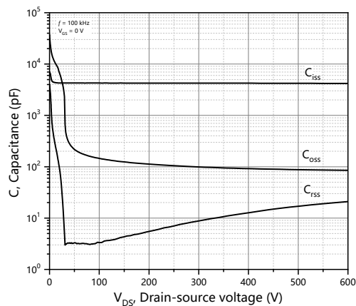
Figure 3. Typ. capacitances
