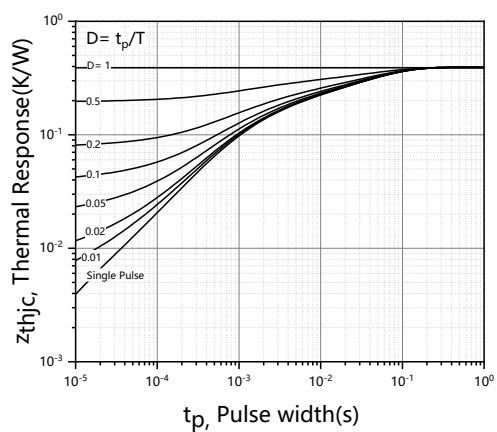
Figure 13. Max. transient thermal impedance
