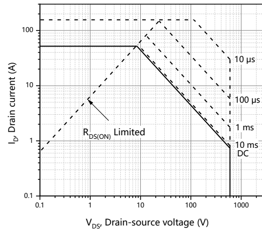
Figure 12. Safe operation area for T_C=25^\circ\text{C}
