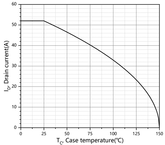
Figure 10. Drain current
