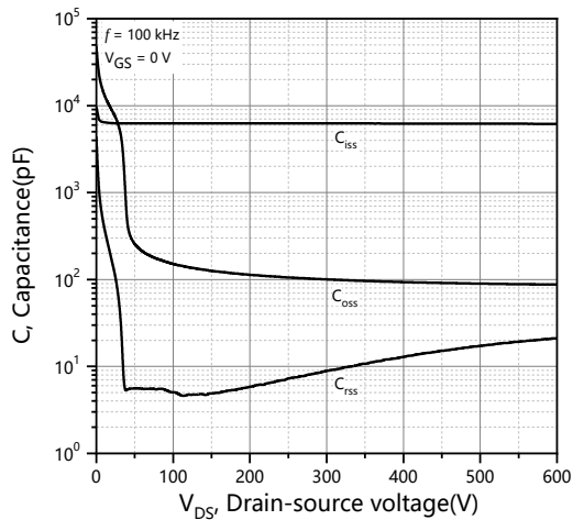
Figure 3. Typ. capacitances
