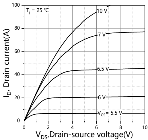
Figure 1. Typ. output characteristics T_j=25^{\circ}\text{C}
