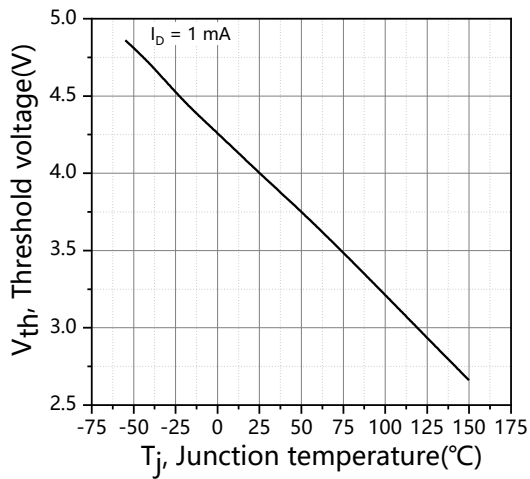
Figure 7. Threshold voltage
