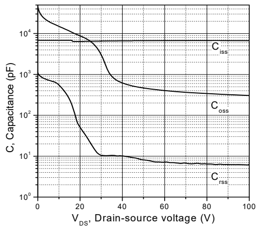
Figure 3. Typ. capacitances
