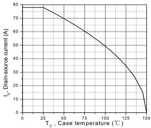
Figure 9. Drain current
