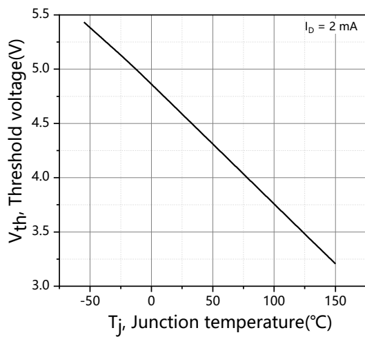
Figure 7. Threshold voltage
