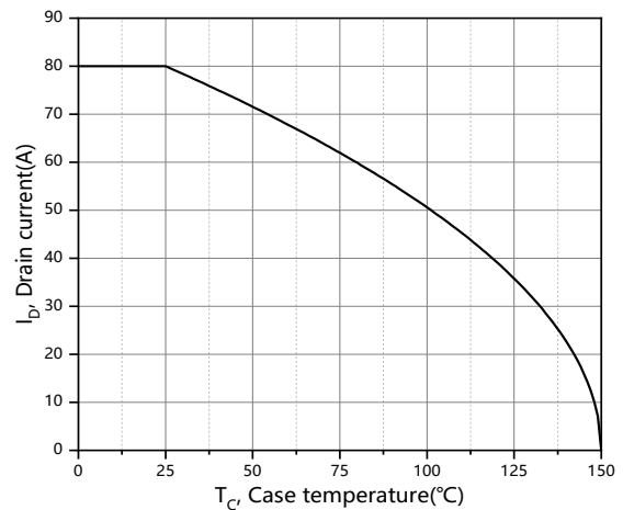
Figure 10. Drain current
