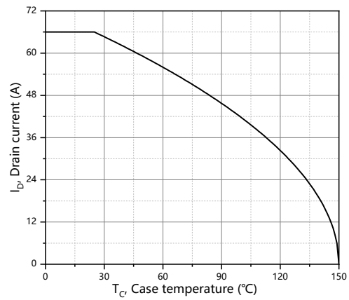
Figure 10. Drain current
