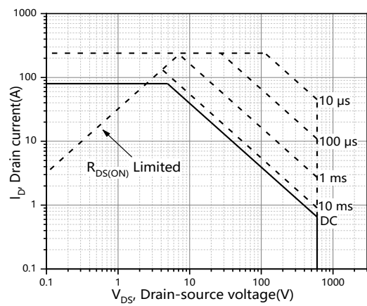
Figure 12. Safe operation area T_C=25 °C
