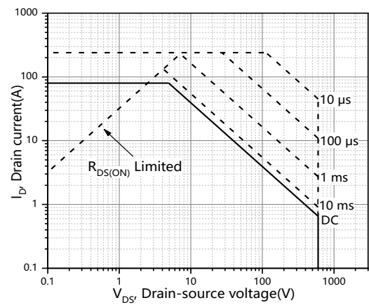
Figure 12. Safe operation area T_c=25\text{ }^{\circ}\text{C}
