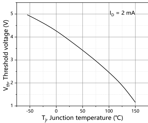
Figure 7. Threshold voltage
