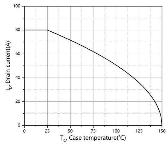
Figure 10. Drain current
