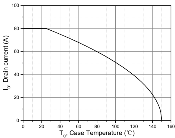
Figure 9. Drain current
