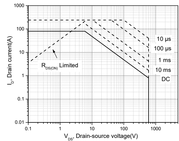
Figure 10. Safe operation area T_c=25\text{ }^{\circ}\text{C}
