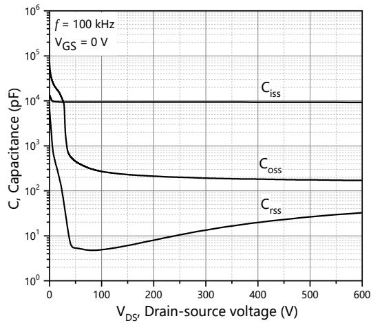
Figure 3. Typ. capacitances
