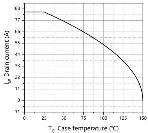
Figure 10. Drain current
