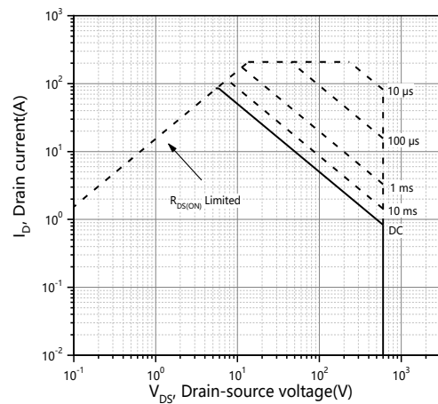
Figure 12. Safe operation area T_c=25\text{°C}
