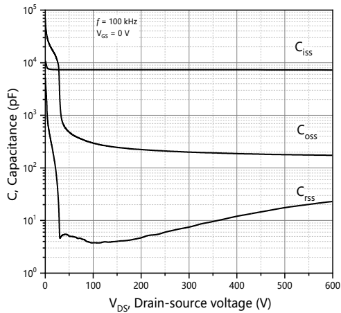
Figure 3. Typ. capacitances
