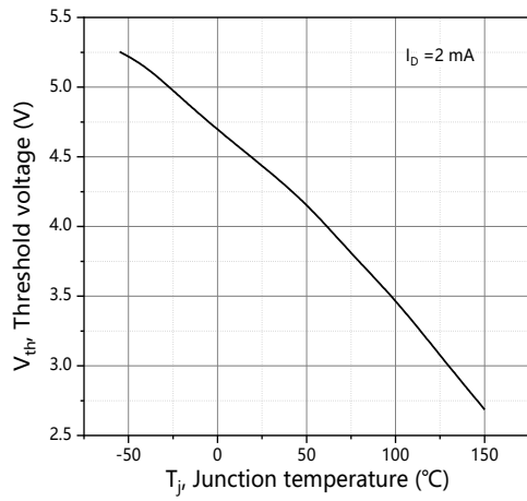
Figure 7. Threshold voltage
