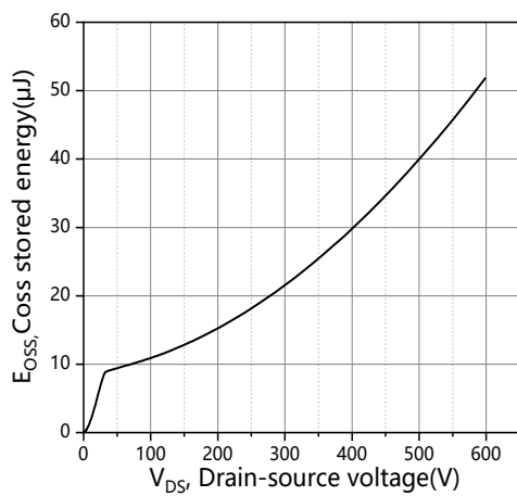
Figure 11. Typ. Coss stored energy
