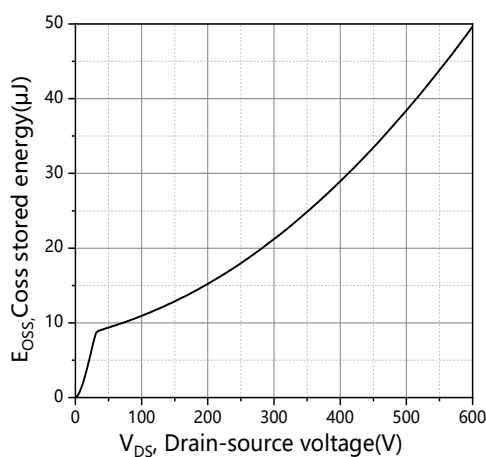
Figure 11. Typ. Coss stored energy
