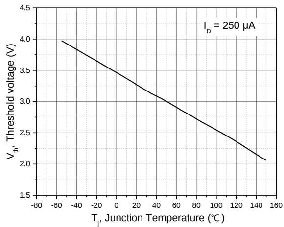
Figure 7. Threshold voltage
