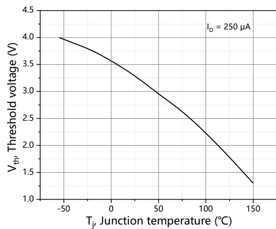
Figure 8. Threshold voltage
