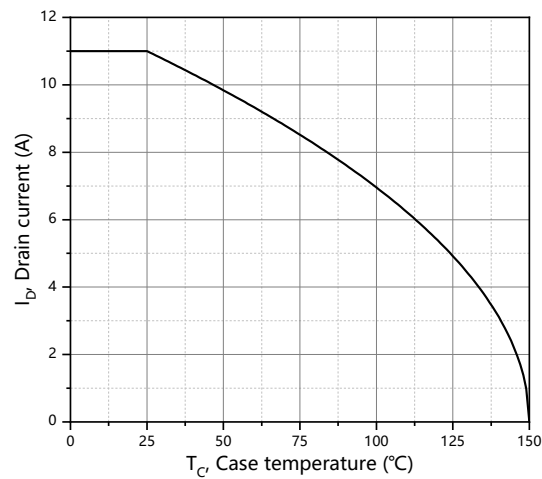
Figure 9. Drain current
