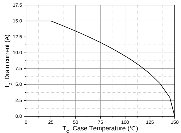
Figure 10. Drain current
