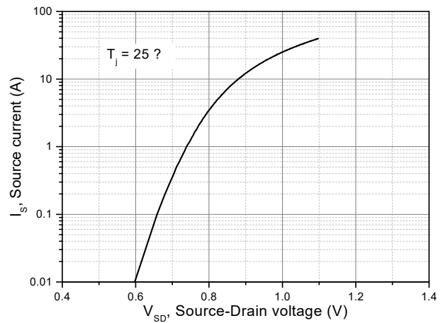
Figure 8. Forward characteristic of body diode
