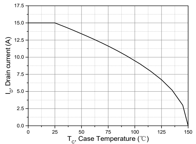
Figure 10. Drain current
