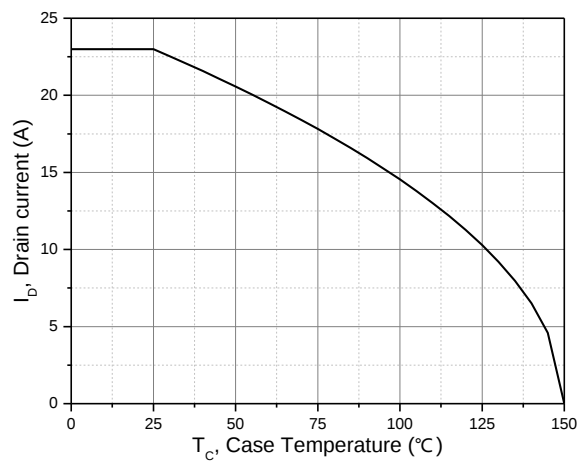
Figure 9. Drain current
