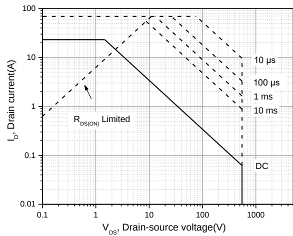
Figure 10. Safe operation area for T_C=25\text{ }^{\circ}\text{C}
