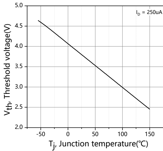
Figure 7. Threshold voltage
