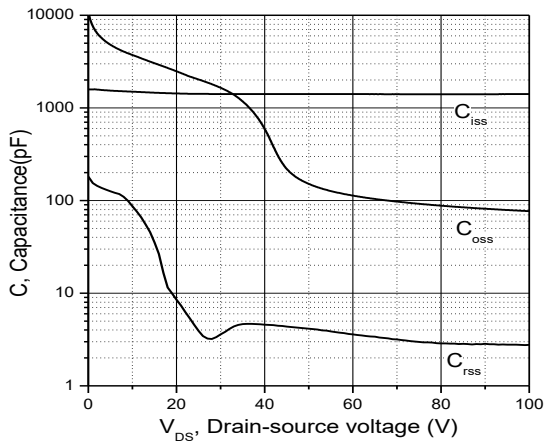
Figure 3. Typ. capacitances
