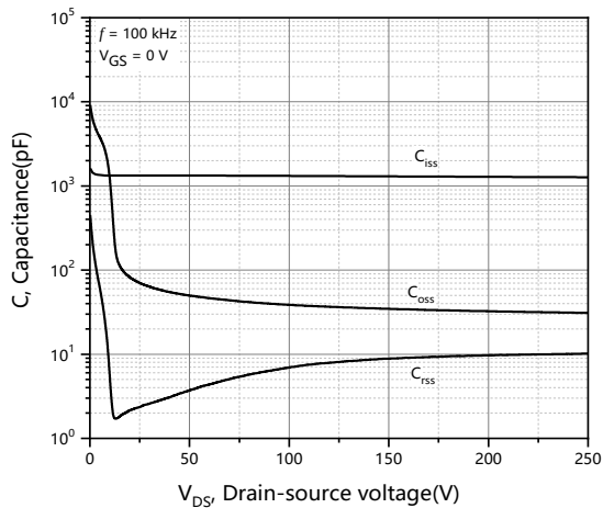
Figure 3. Typ. capacitances
