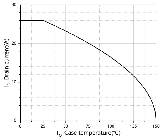
Figure 10. Drain current
