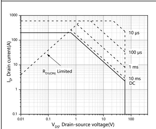
Figure 11. Safe operation area for T_c=25^\circ C
