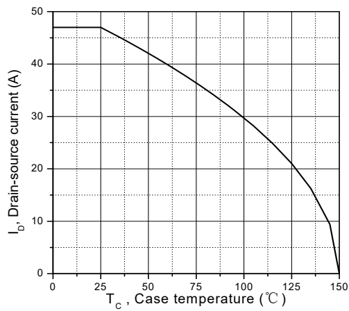
Figure 9. Drain current
