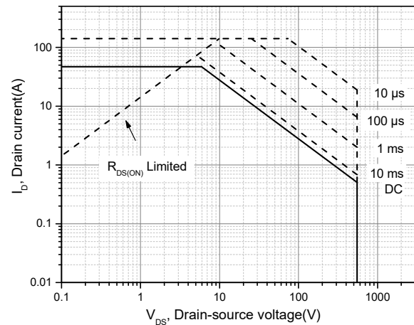
Figure 10. Safe operation area Tc=25 °C
