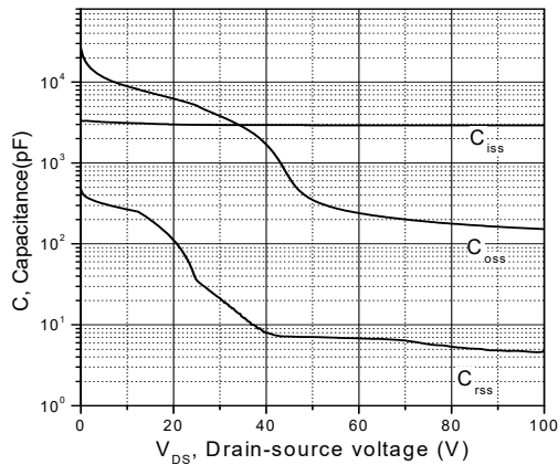
Figure 3. Typ. capacitances
